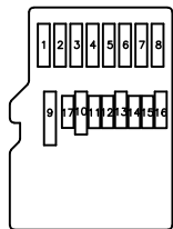
Micro SD 4.0 CARD
