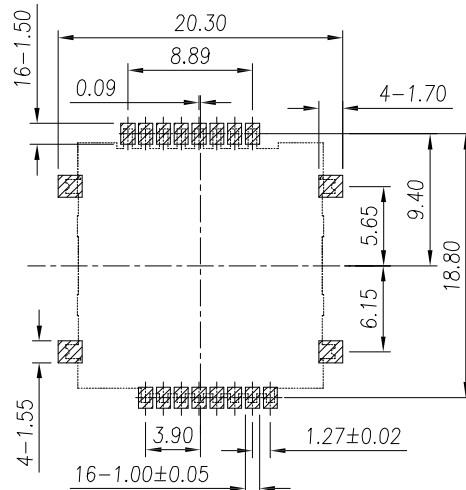
RECOMMENDED P.C.B LAYOUT GENERAL TOLERANCE ± 0.05
