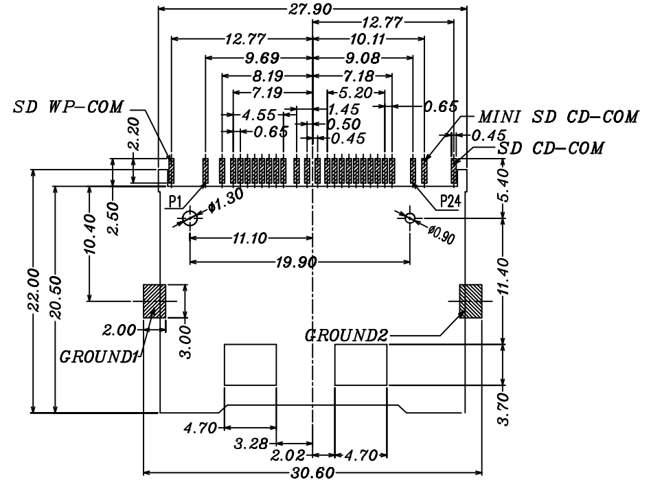
RECOMMENDED P.C.B. LAYOUT (General tolerance \pm 0.05 )
