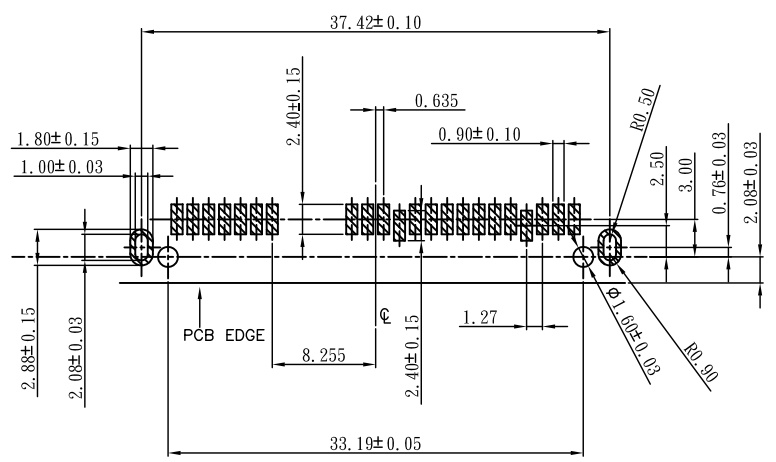
RECOMMEND PCB LAYOUT (T=1.2) PCB TOLERANCE:±0.05
