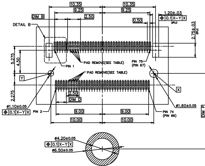
RECOMMENDED NGFF PCB LAYOUT
