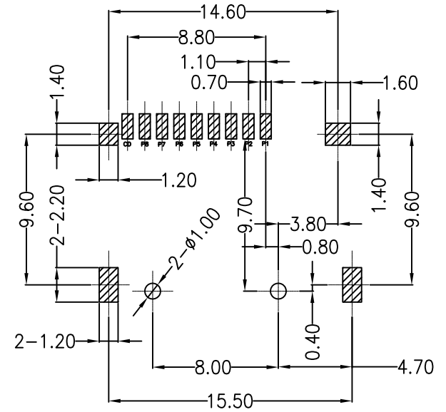
P.C.B. LAYOUT (TOLERANCE±0.05)
