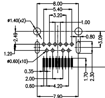
P.C.B LAYOUT (T=1.60mm) VIEW BOTTOM (tolerance±0.05)
