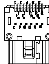
P.C.B LAYOUT (T=1.60mm) VIEW BOTTOM (tolerance±0.05)
