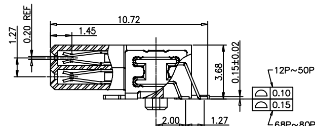
CROSS SECTION SCALE 2:1
