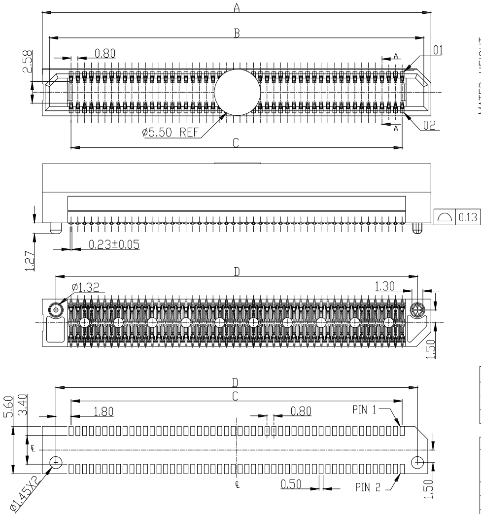
Recommended PC board pattern (TOP VIEW)
